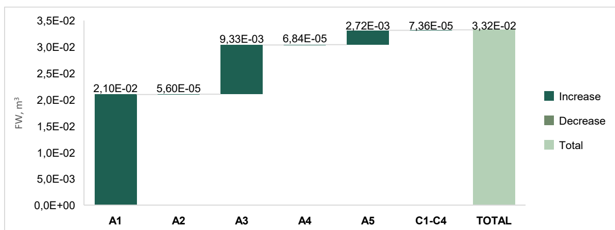
Net freshwater use for 1 m 2 of installed Norgips FLOOR 12.5mm gypsum plasterboard
