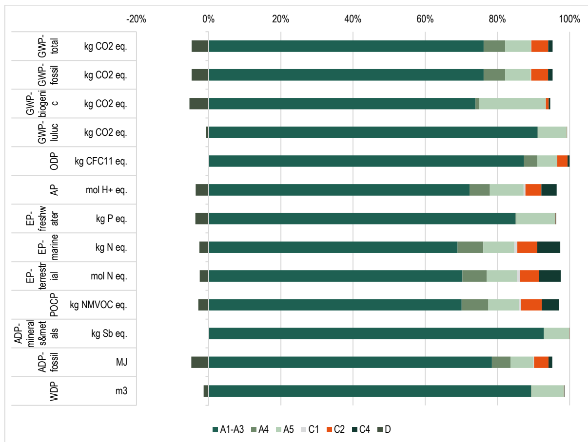
Contribution to environmental impact per each module for 1 m 2 of installed Norgips FLOOR 12.5mm gypsum plasterboard
