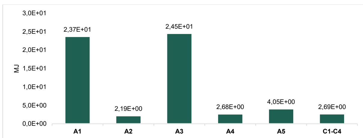
Primary energy demand per 1 m 2 of installed Norgips FLOOR 12.5mm gypsum plasterboard
